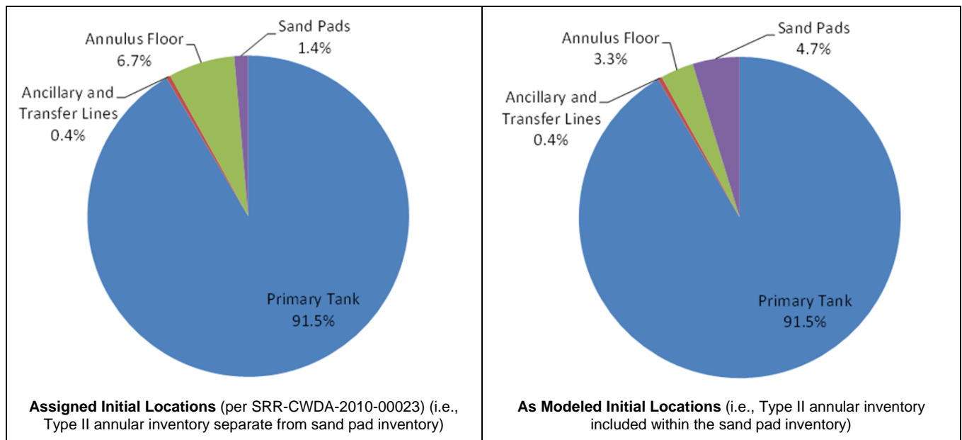
Figure CQ-2.2: Comparison of Total Initial Curies of Sr-90 for All HTF Sources
