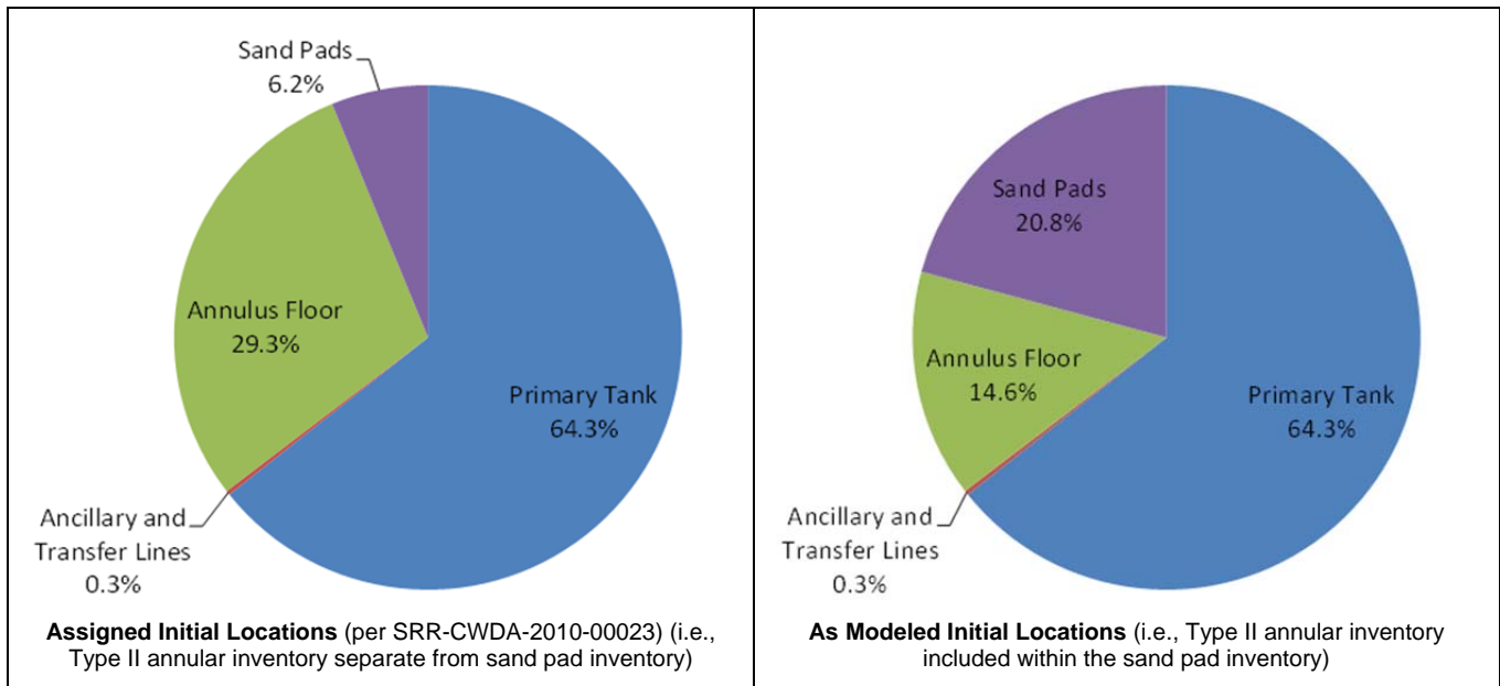
Figure CQ-2.1: Comparison of Total Initial Curies of Cs-137 for All HTF Sources
